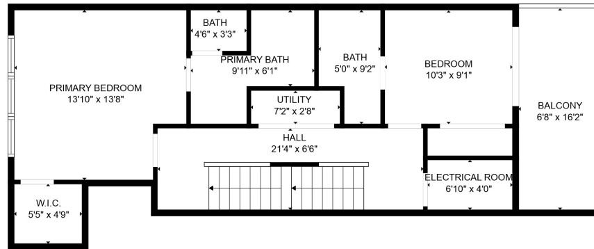
FLOOR 2
